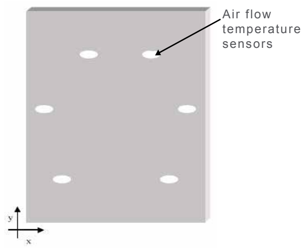
Figure 1: Sensor locations on a 6U x 160mm board
