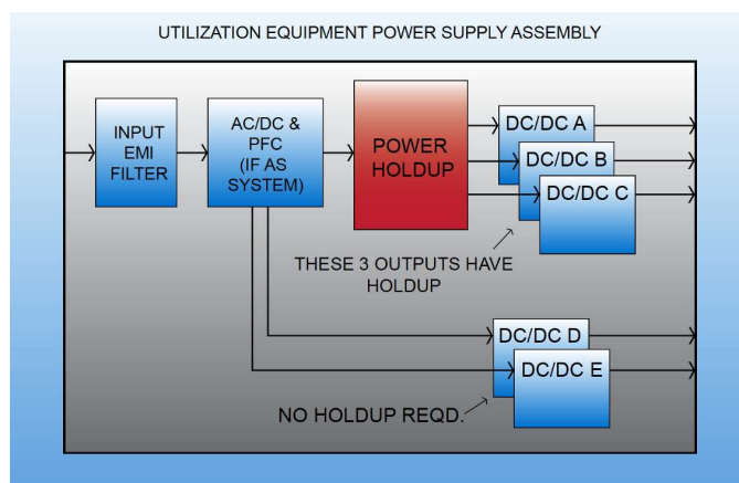
Typical Holdup Function Within System Power Supply
